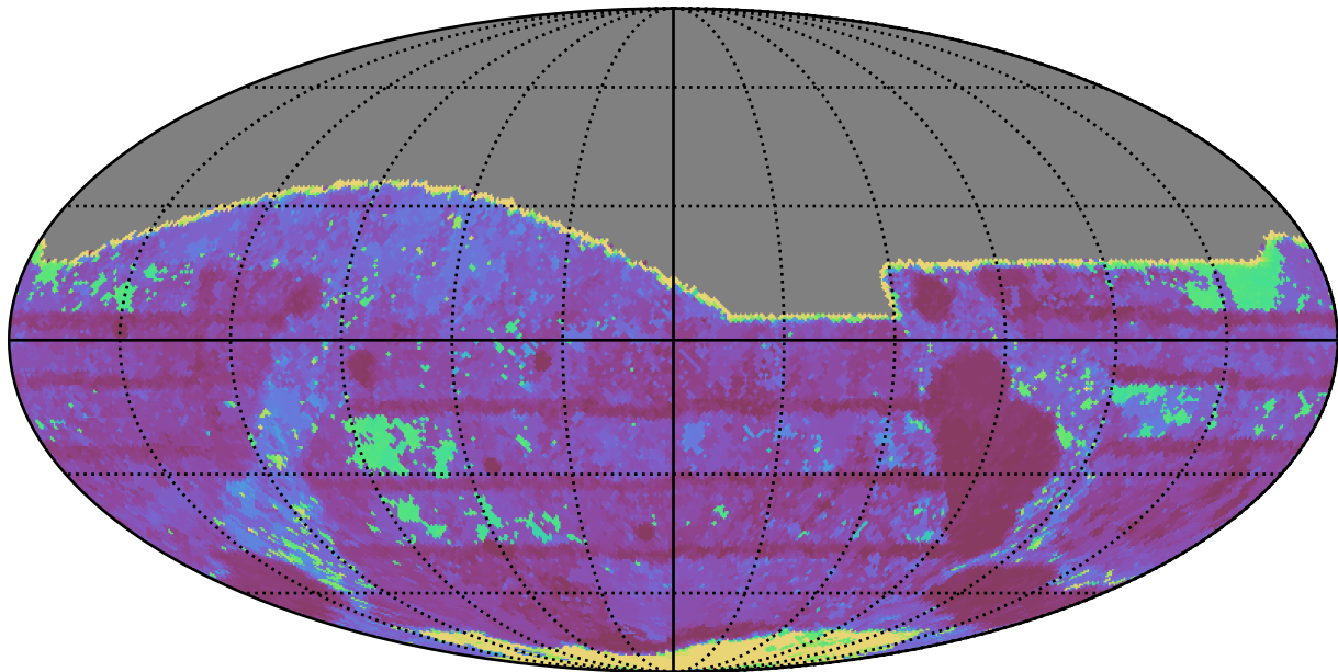
too_10_4v3.4_10yrs All sky r band: Max Inter-Night Gap
