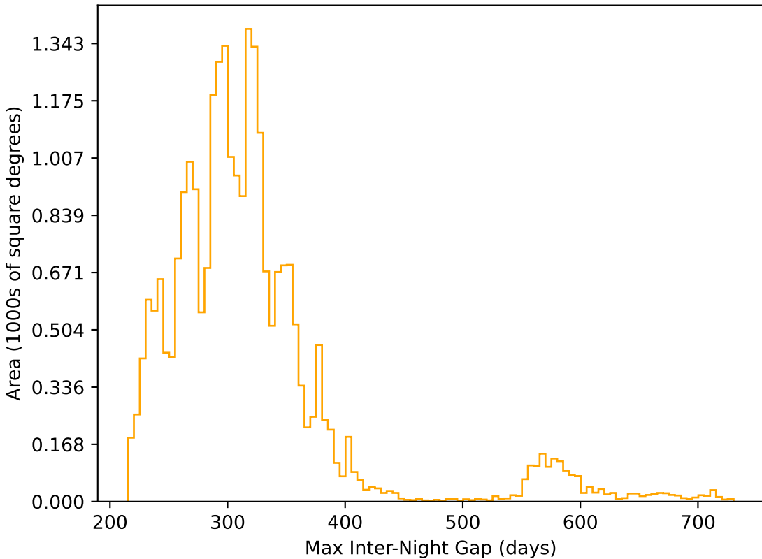
too_10_4v3.4_10yrs All sky r band: Max Inter-Night Gap
