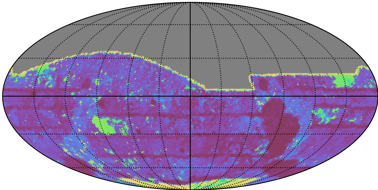
too_10_4v3.4_10yrs All sky i band: Max Inter-Night Gap
