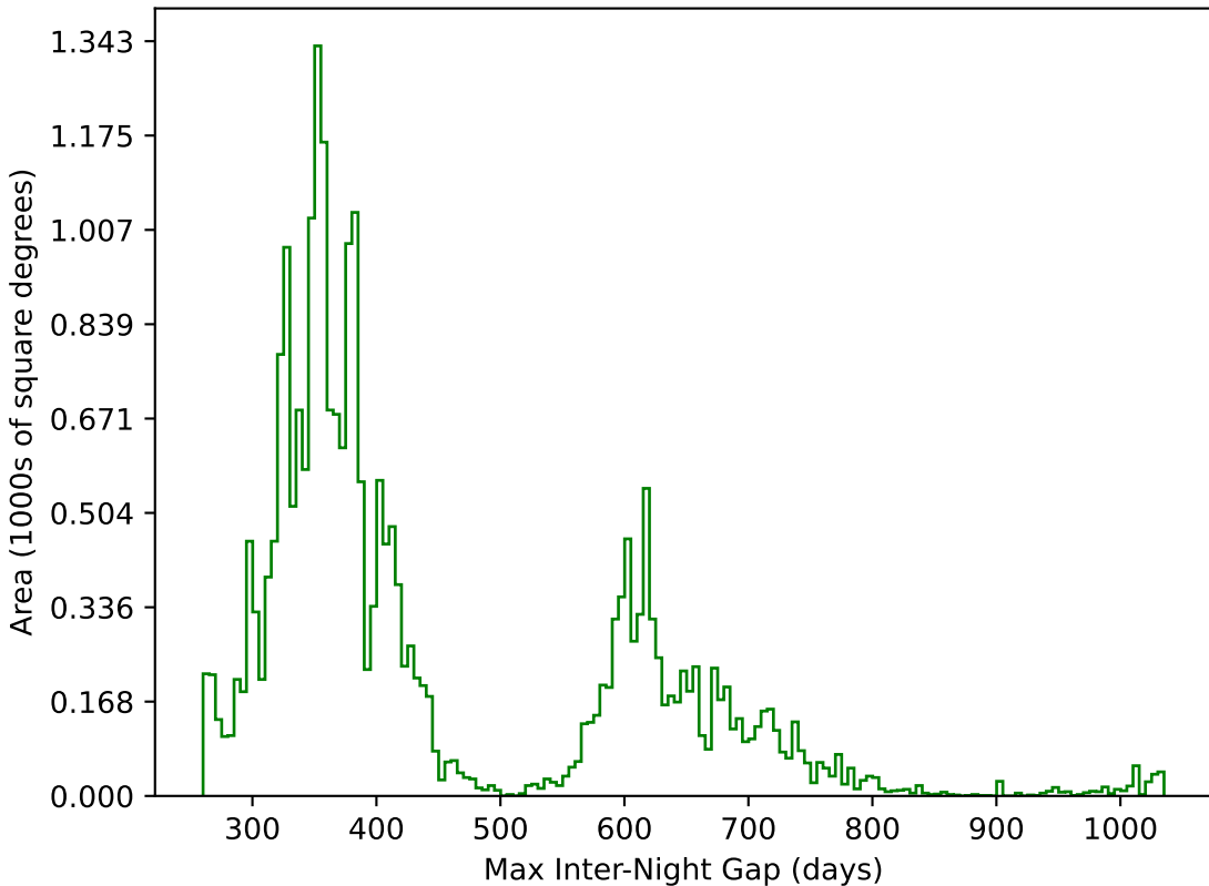
too_10_4v3.4_10yrs All sky g band: Max Inter-Night Gap
