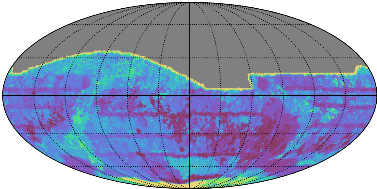
too_10_4v3.4_10yrs All sky all bands: Max Inter-Night Gap
