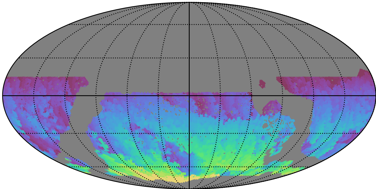
too_10_4v3.4_10yrs WFD z band: Max HA
