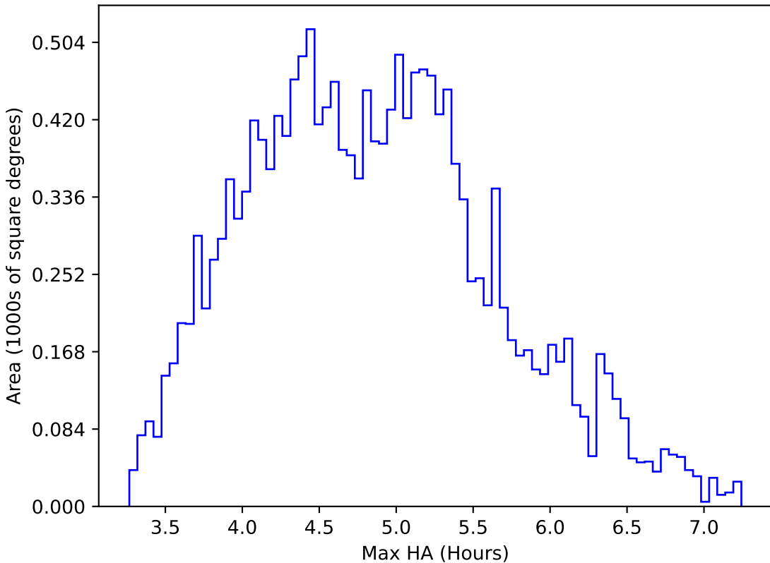
too_10_4v3.4_10yrs WFD z band: Max HA
