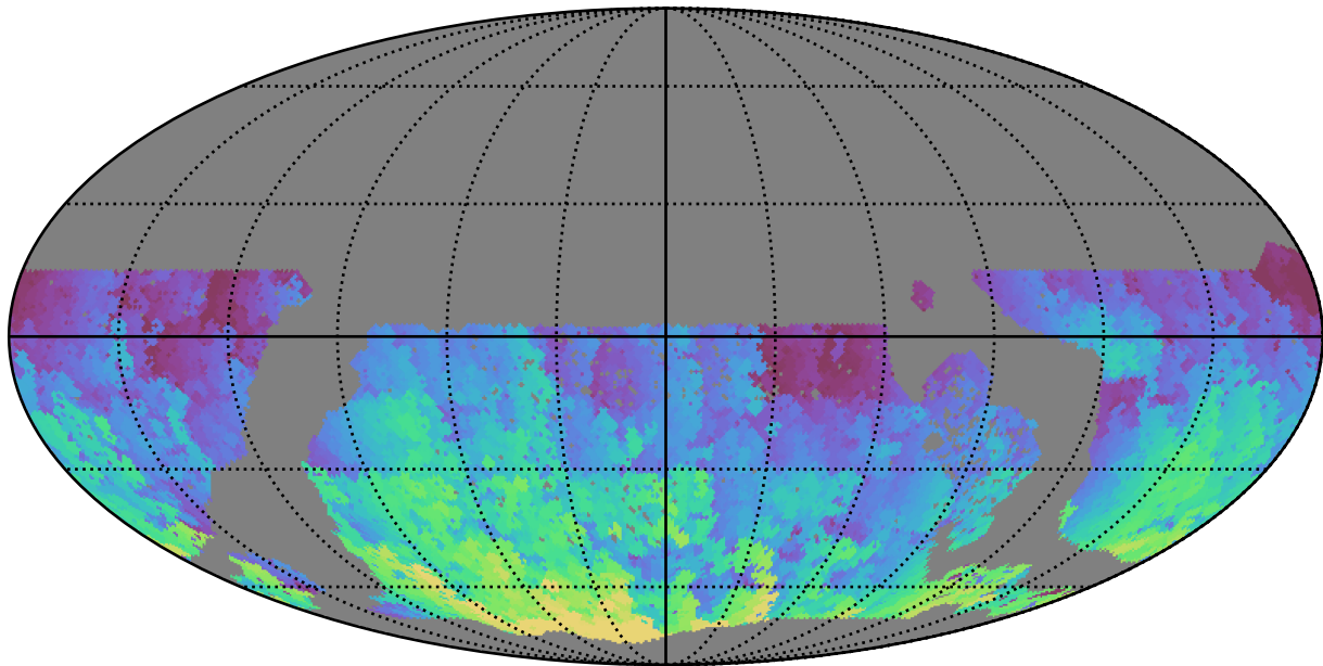
too_10_4v3.4_10yrs WFD u band: Max HA
