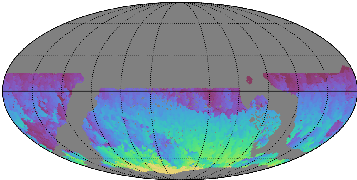
too_10_4v3.4_10yrs WFD i band: Max HA
