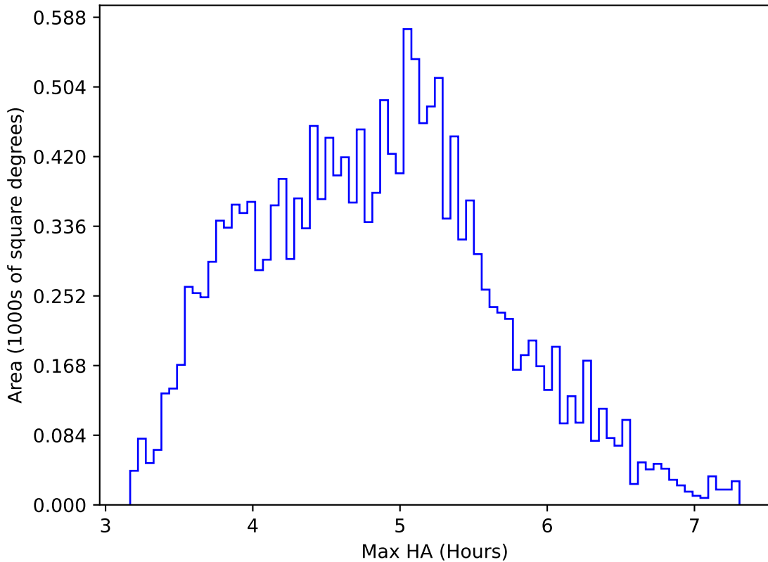
too_10_4v3.4_10yrs WFD i band: Max HA
