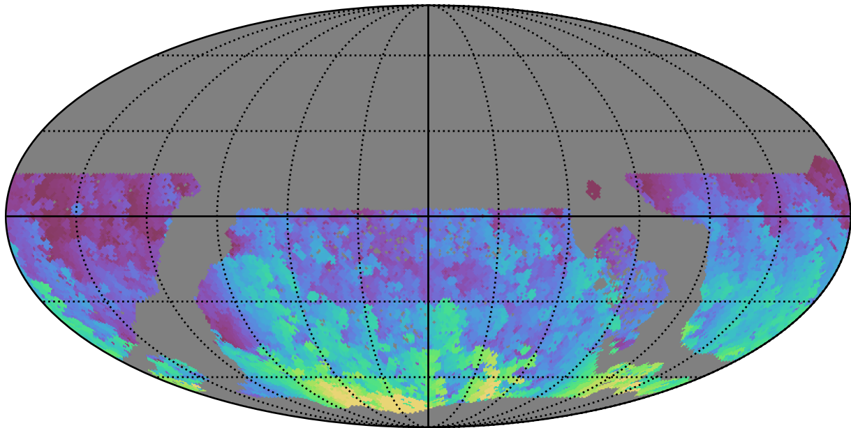
too_10_4v3.4_10yrs WFD g band: Max HA
