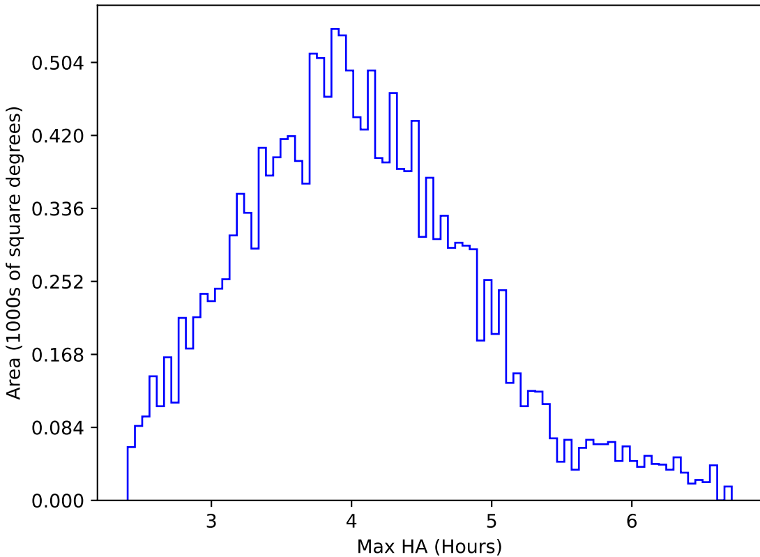
too_10_4v3.4_10yrs WFD g band: Max HA
