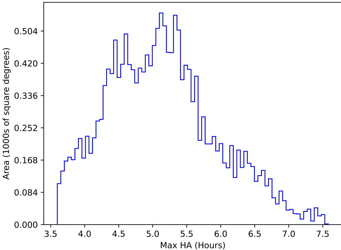
too_10_4v3.4_10yrs WFD all bands: Max HA
