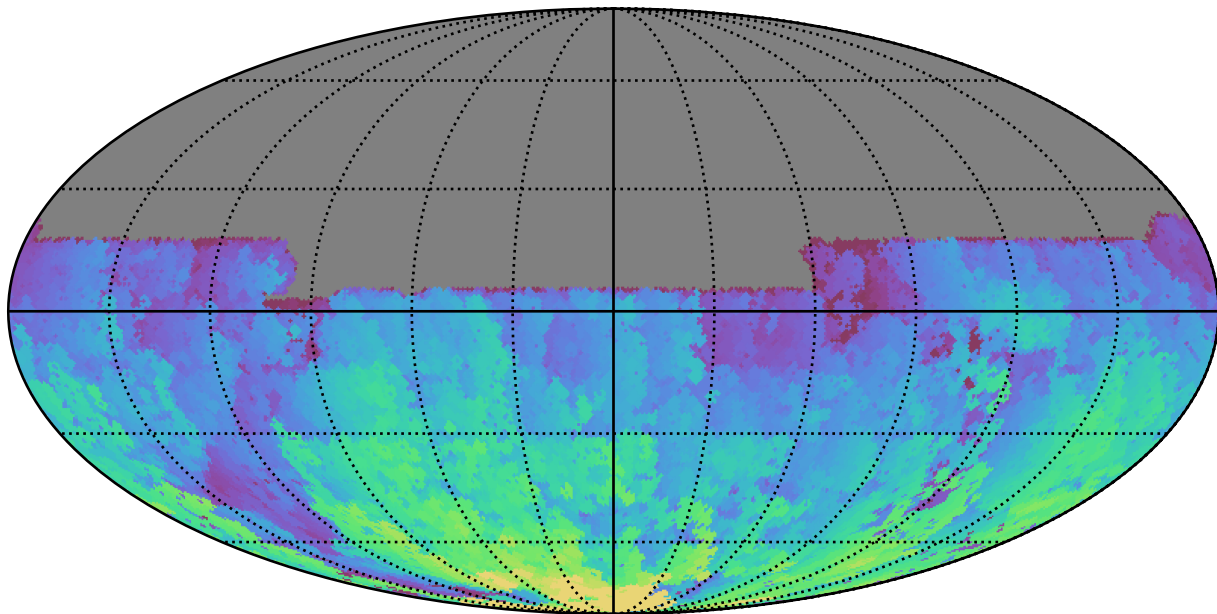
too_10_4v3.4_10yrs All sky u band: Max HA
