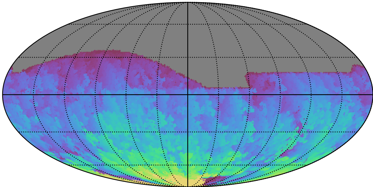
too_10_4v3.4_10yrs All sky r band: Max HA
