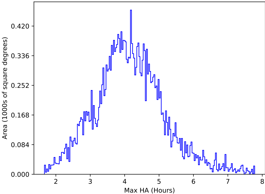
too_10_4v3.4_10yrs All sky r band: Max HA
