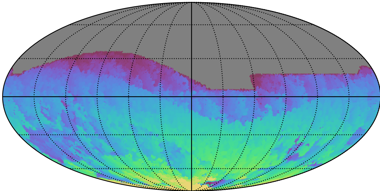
too_10_4v3.4_10yrs All sky i band: Max HA
