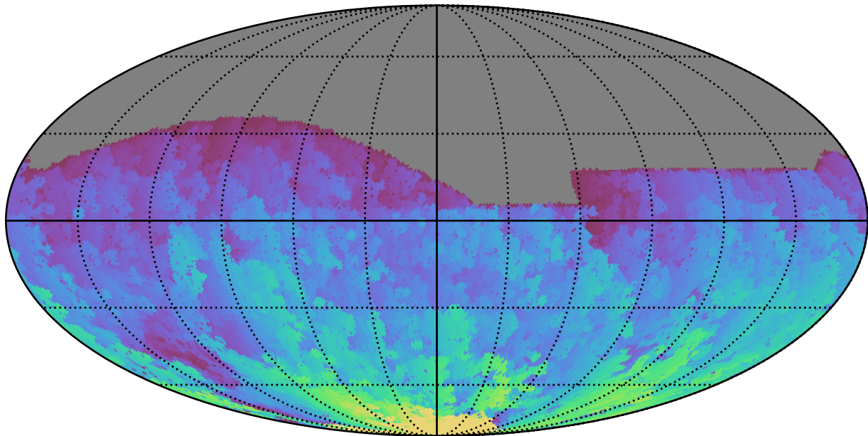
too_10_4v3.4_10yrs All sky g band: Max HA
