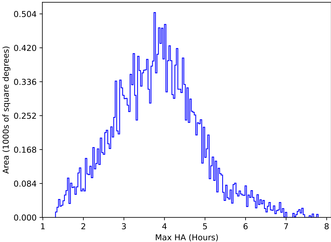
too_10_4v3.4_10yrs All sky g band: Max HA
