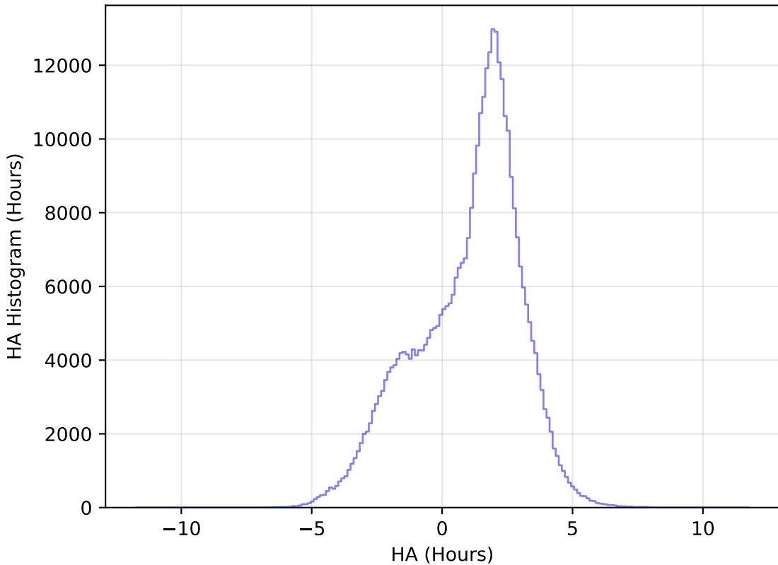
too_10_4v3.4_10yrs WFD y band: HA Histogram
