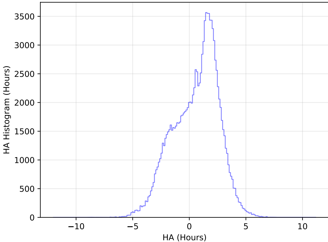
too_10_4v3.4_10yrs WFD u band: HA Histogram
