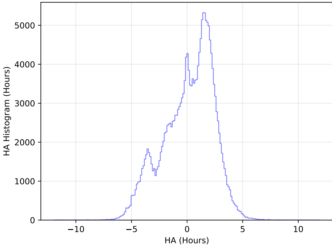
too_10_4v3.4_10yrs WFD g band: HA Histogram
