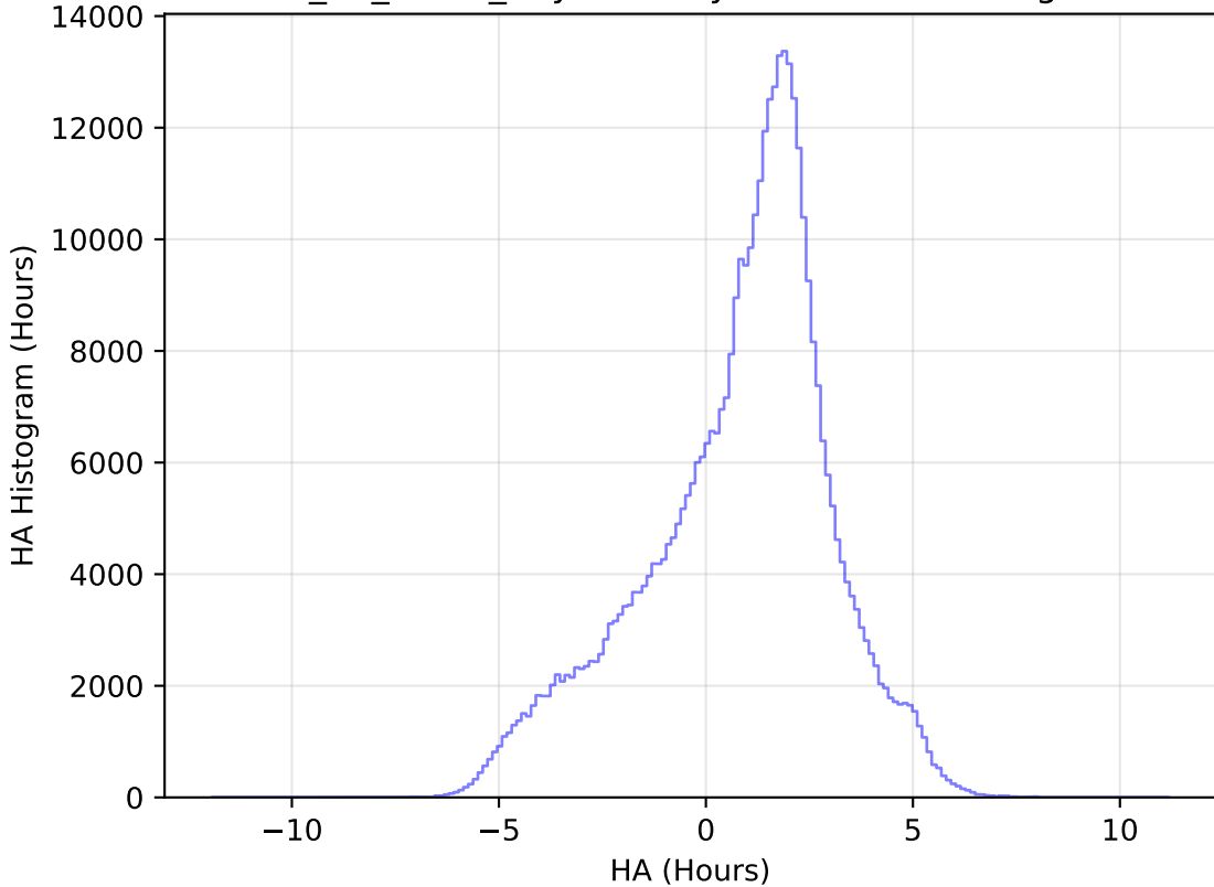
too_10_4v3.4_10yrs All sky z band: HA Histogram
