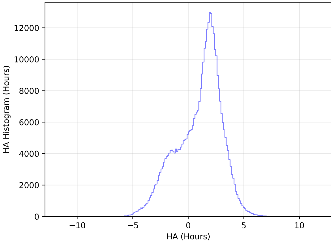
too_10_4v3.4_10yrs All sky y band: HA Histogram
