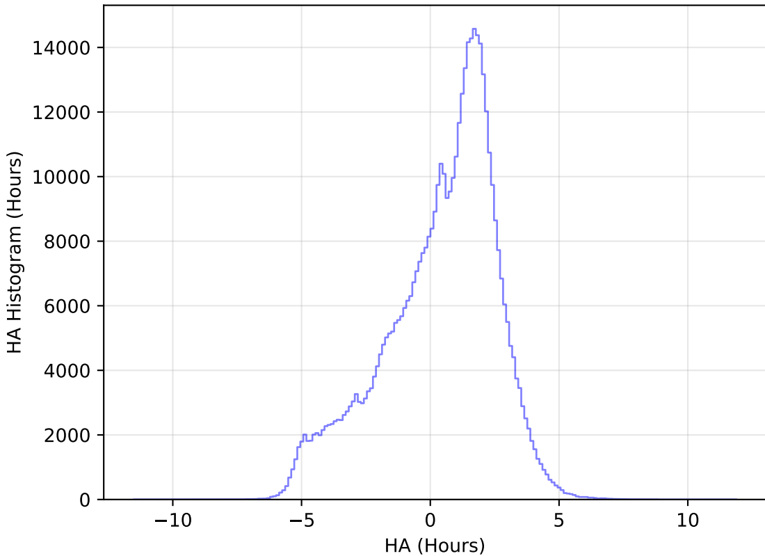
too_10_4v3.4_10yrs All sky r band: HA Histogram
