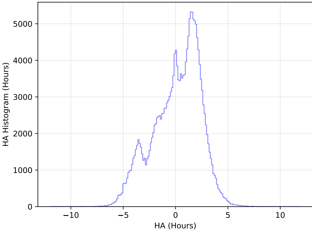
too_10_4v3.4_10yrs All sky g band: HA Histogram
