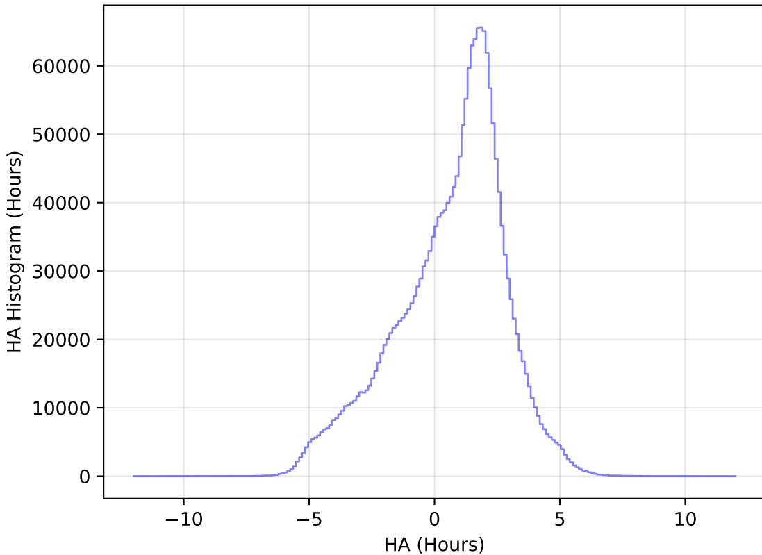
too_10_4v3.4_10yrs All sky all bands: HA Histogram
