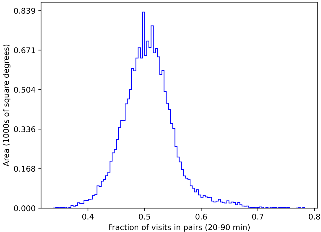
too_10_4v3.4_10yrs gri WFD: Fraction of visits in pairs (20-90 min)
