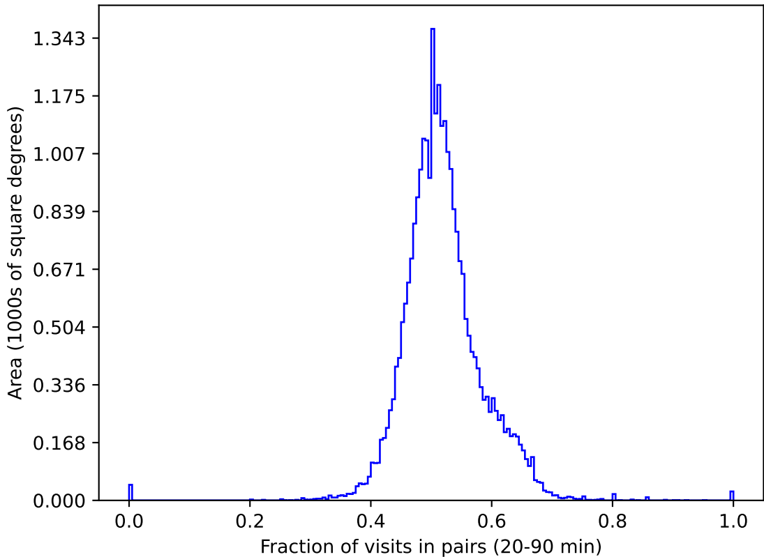
too_10_4v3.4_10yrs gri All sky: Fraction of visits in pairs (20-90 min)
