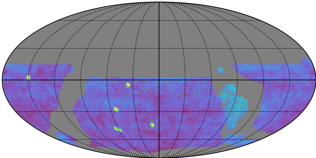
too_10_4v3.4_10yrs gri WFD: Fraction of visits in pairs (10-60 min)
