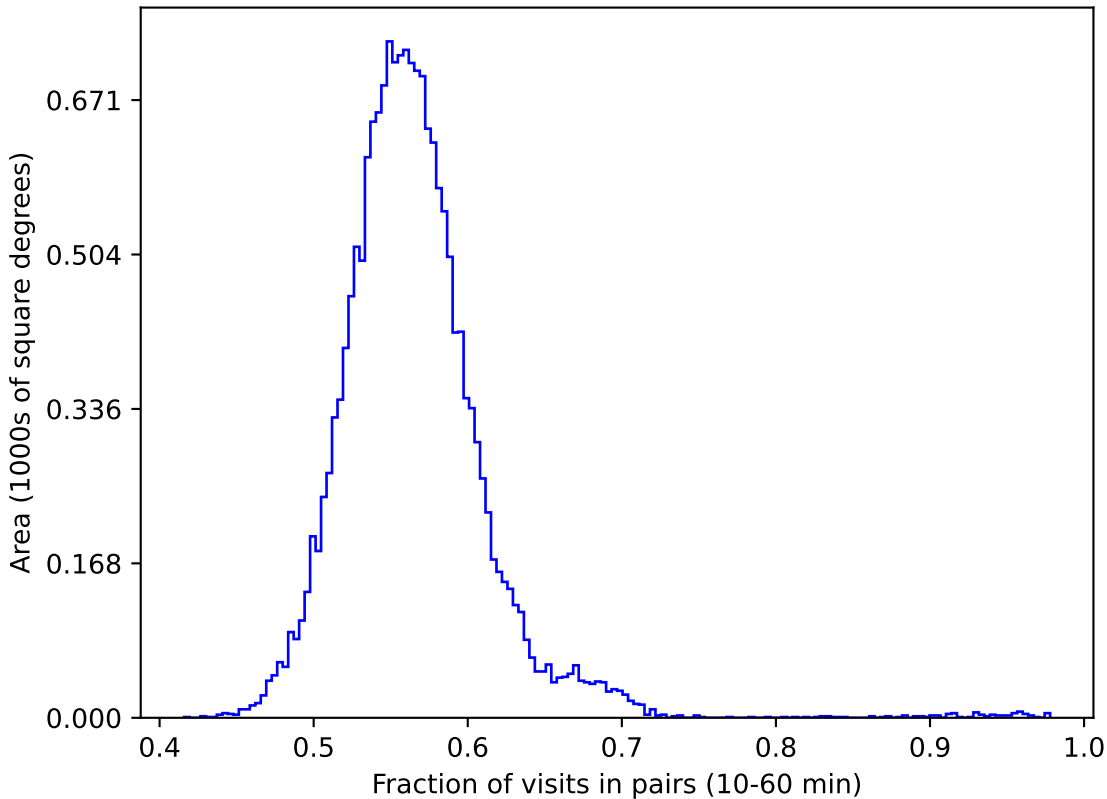
too_10_4v3.4_10yrs gri WFD: Fraction of visits in pairs (10-60 min)
