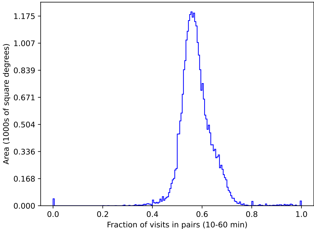
too_10_4v3.4_10yrs gri All sky: Fraction of visits in pairs (10-60 min)
