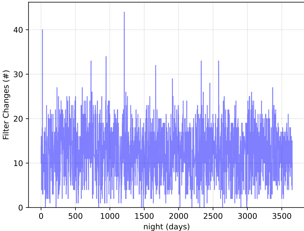
too_10_4v3.4_10yrs Per Night: Filter Changes
