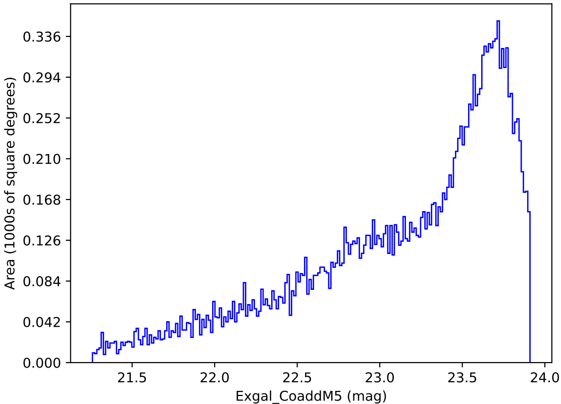
too_10_4v3.4_10yrs Yr 3-4 y band: Exgal_CoaddM5
