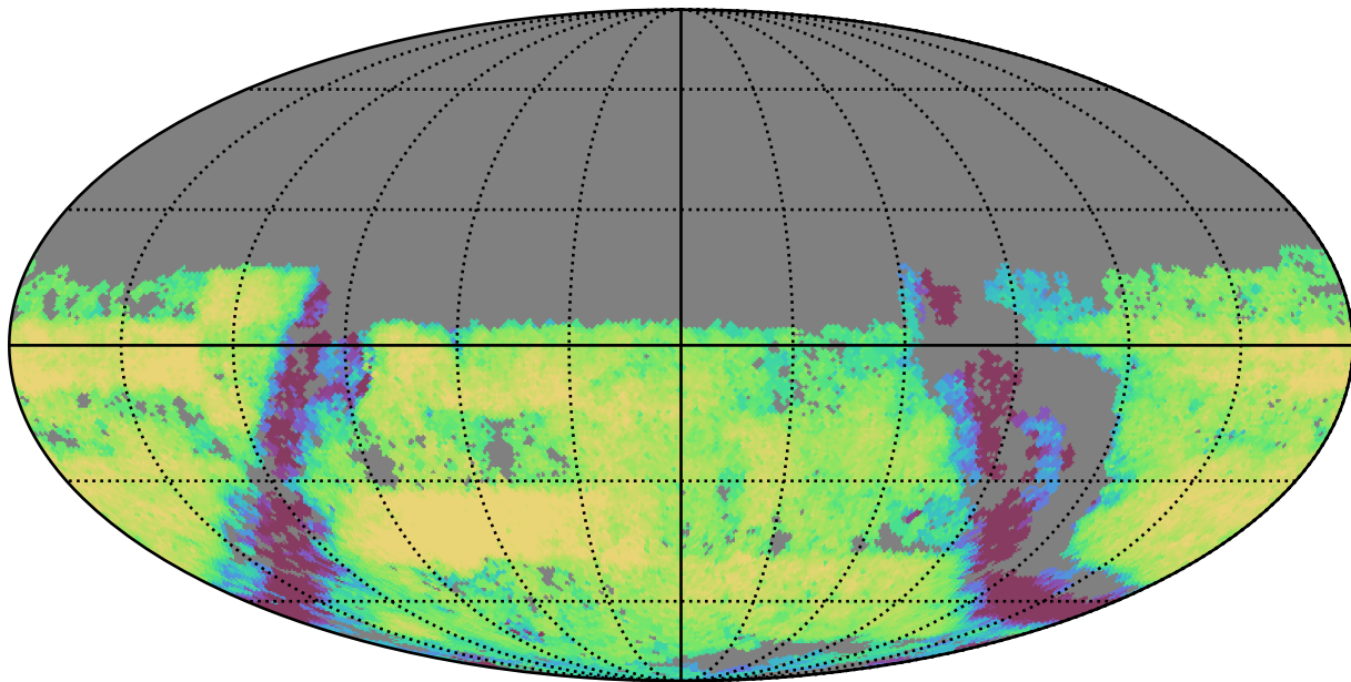
too_10_4v3.4_10yrs Yr 3-4 u band: Exgal_CoaddM5
