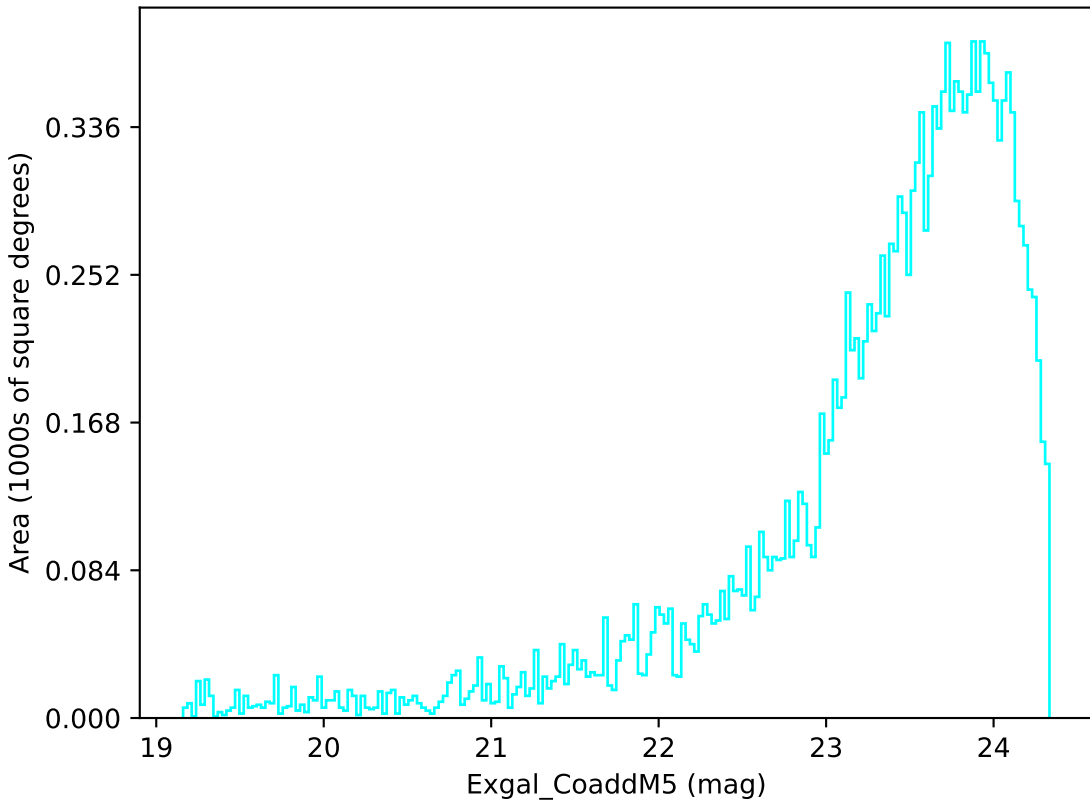
too_10_4v3.4_10yrs Yr 3-4 u band: Exgal_CoaddM5
