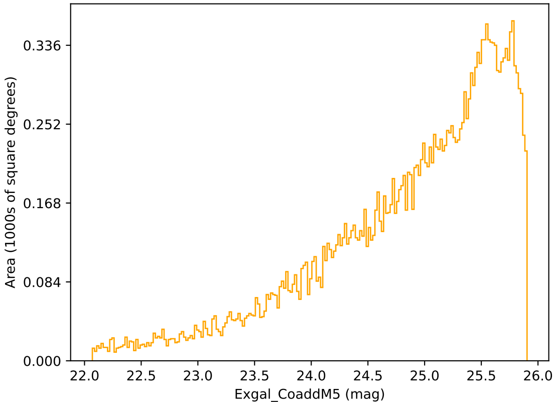
too_10_4v3.4_10yrs Yr 3-4 r band: Exgal_CoaddM5
