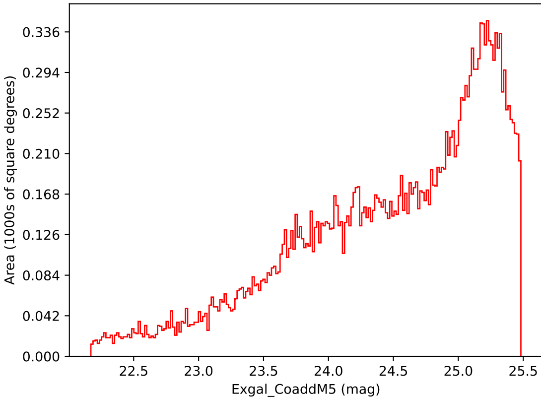
too_10_4v3.4_10yrs Yr 3-4 i band: Exgal_CoaddM5
