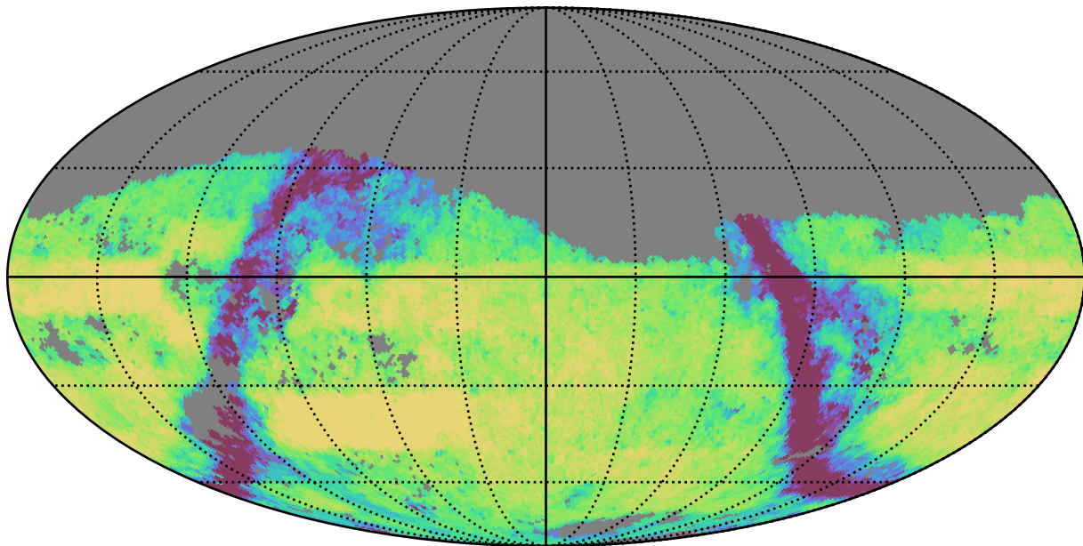
too_10_4v3.4_10yrs Yr 3-4 g band: Exgal_CoaddM5
