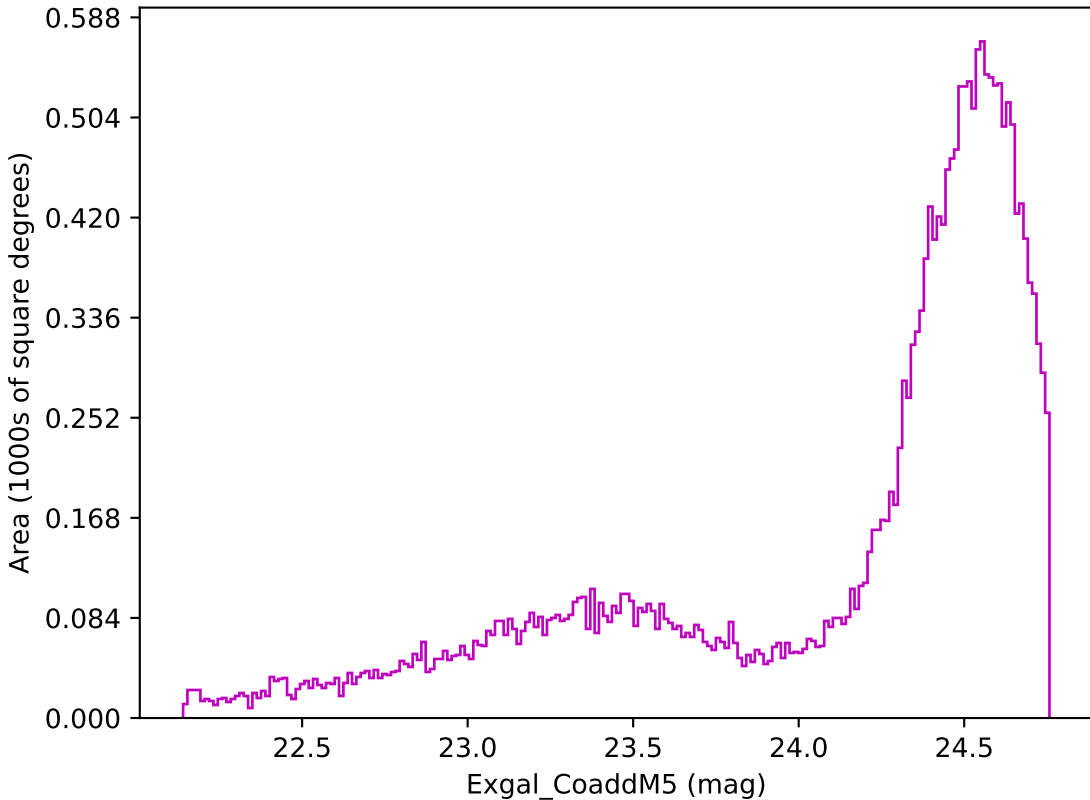
too_10_4v3.4_10yrs Yr 1 z band: Exgal_CoaddM5
