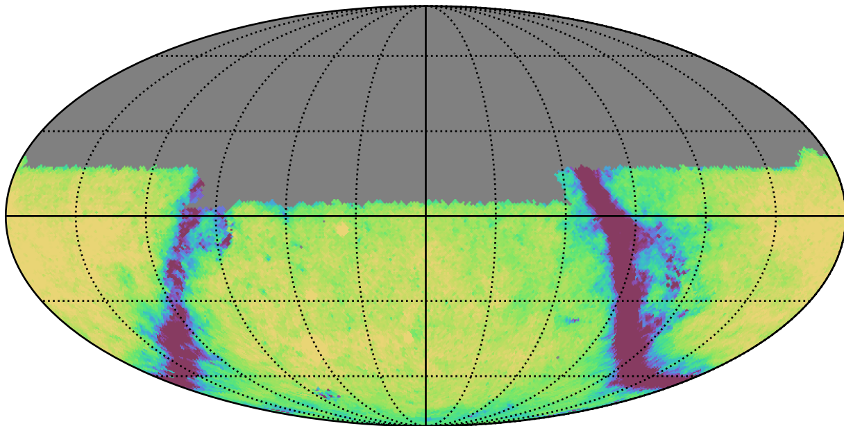
too_10_4v3.4_10yrs Yr 1 u band: Exgal_CoaddM5
