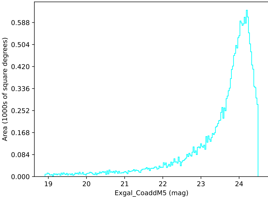
too_10_4v3.4_10yrs Yr 1 u band: Exgal_CoaddM5
