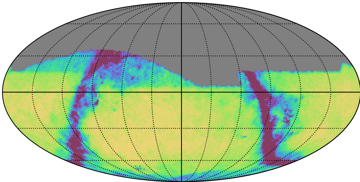
too_10_4v3.4_10yrs Yr 1 r band: Exgal_CoaddM5
