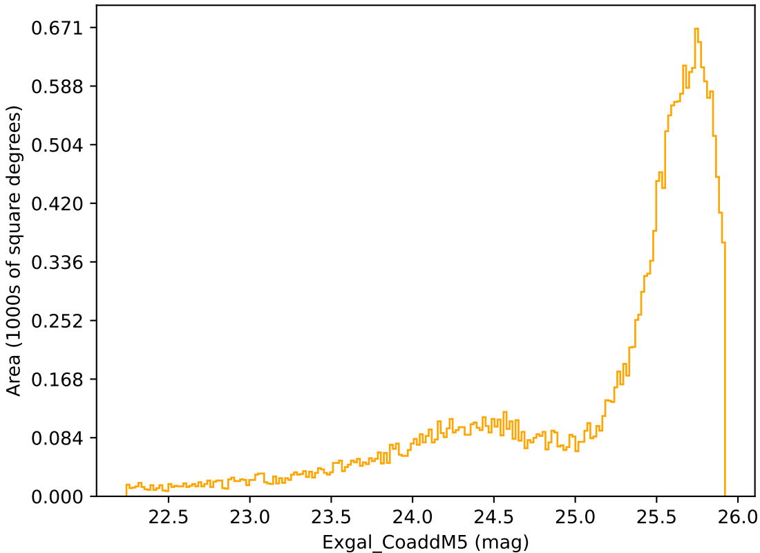
too_10_4v3.4_10yrs Yr 1 r band: Exgal_CoaddM5
