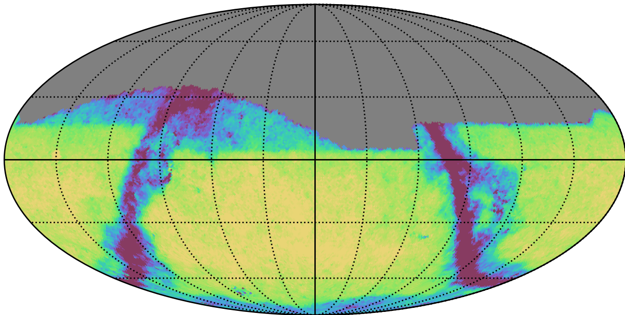
too_10_4v3.4_10yrs Yr 1 i band: Exgal_CoaddM5
