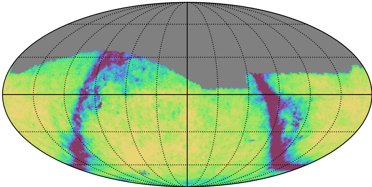
too_10_4v3.4_10yrs Yr 1 g band: Exgal_CoaddM5
