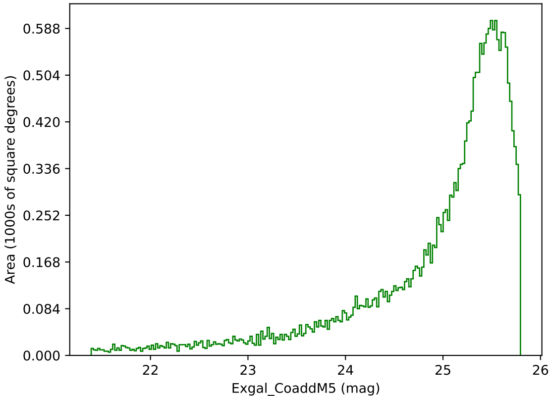
too_10_4v3.4_10yrs Yr 1 g band: Exgal_CoaddM5
