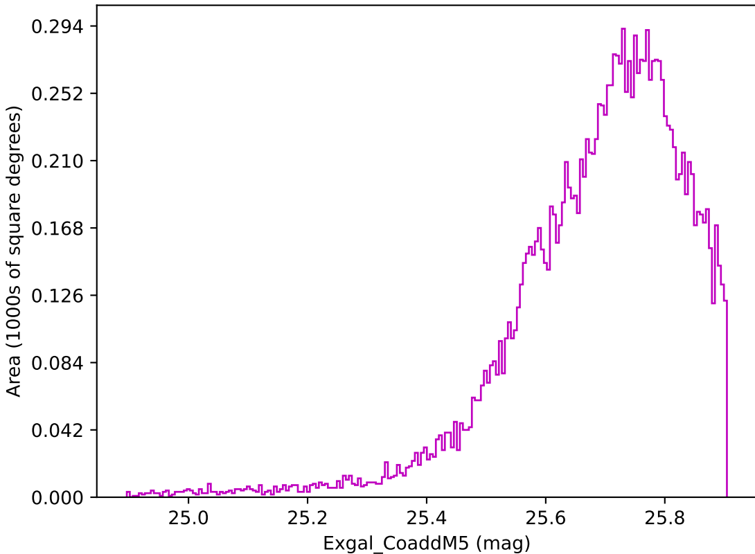
too_10_4v3.4_10yrs WFD z band: Exgal_CoaddM5
