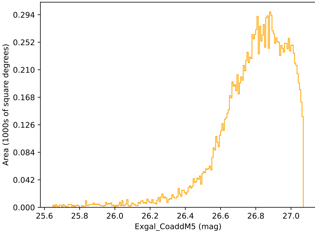
too_10_4v3.4_10yrs WFD r band: Exgal_CoaddM5
