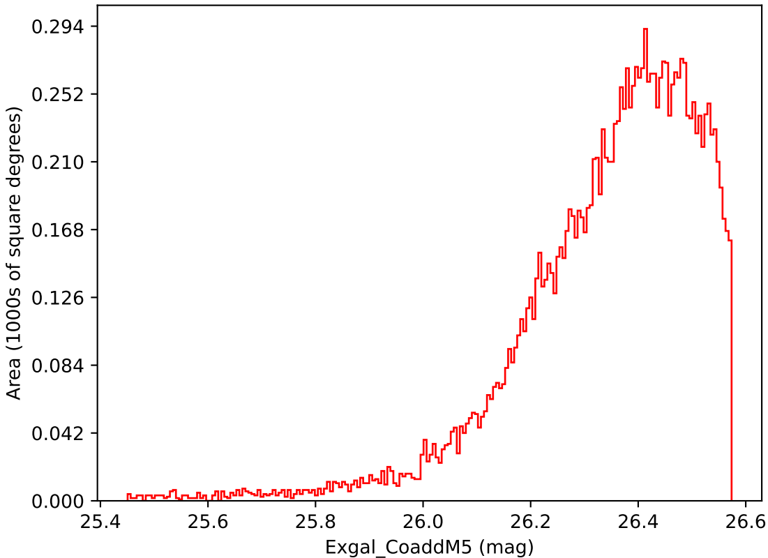
too_10_4v3.4_10yrs WFD i band: Exgal_CoaddM5
